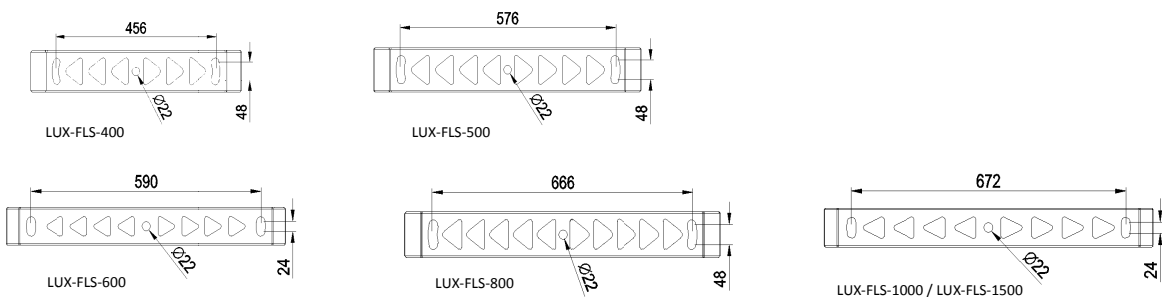
Fig. 1 Measurements of bracket mounting holes
