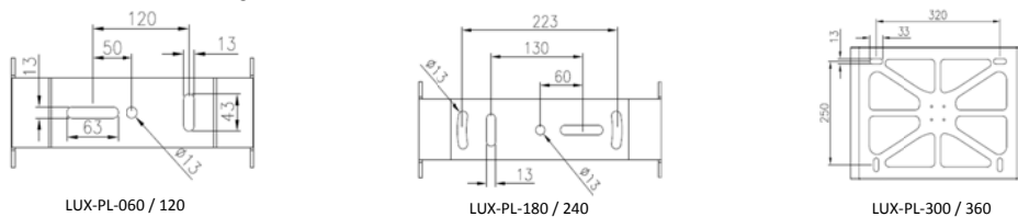
Fig. 1 Measurements of bracket mounting holes
